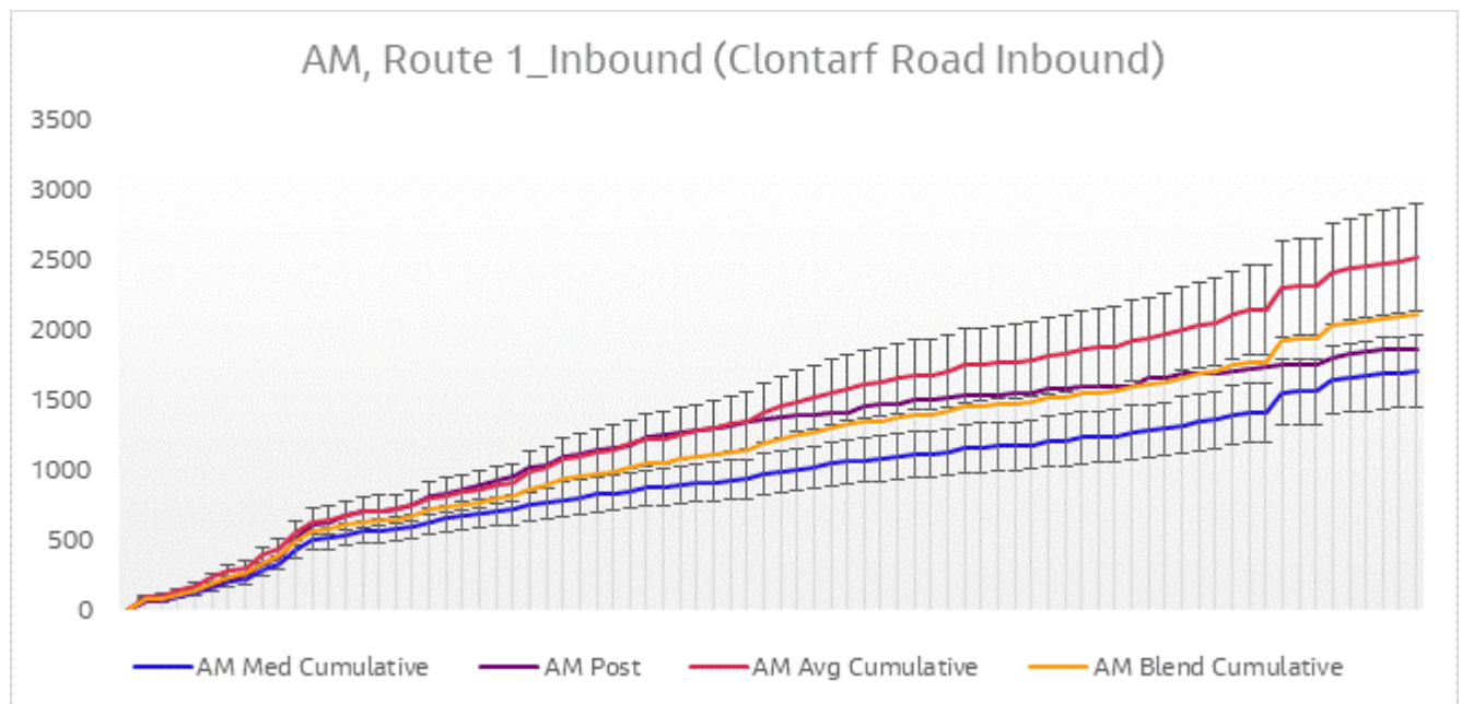
Figure 6-11 Journey Time Validation Plot - Route 1 Inbound AM
