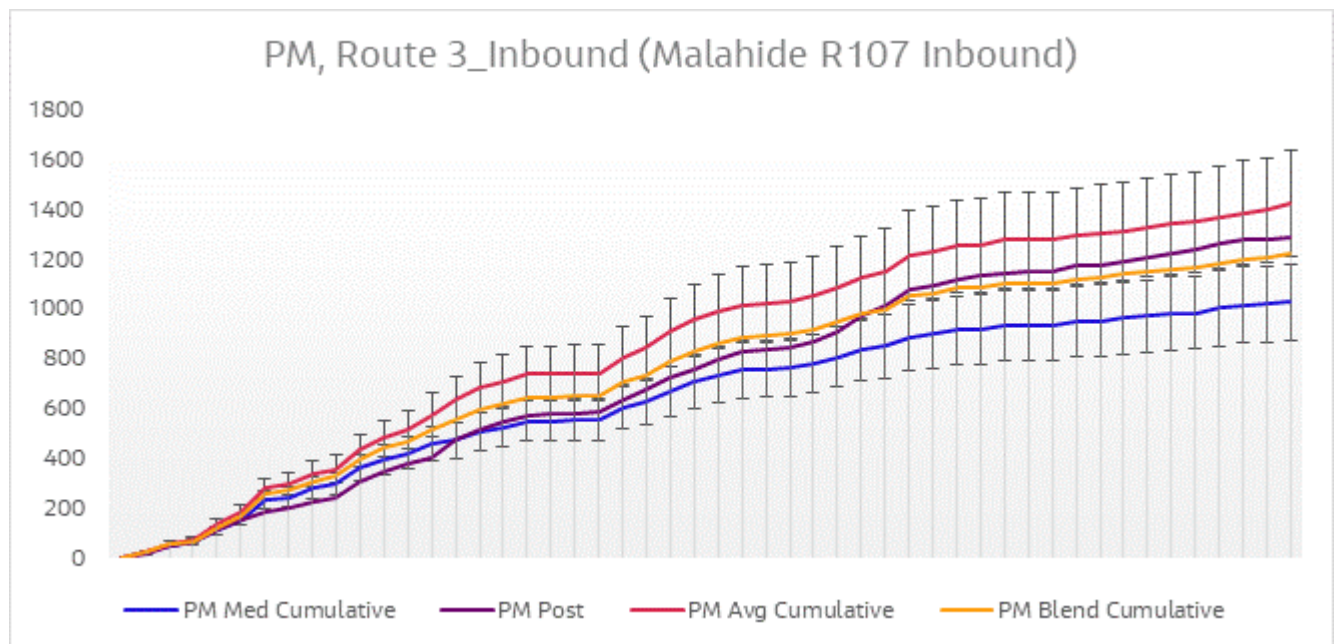
Figure 6-25 Journey Time Validation Plot - Route 3 Inbound PM
