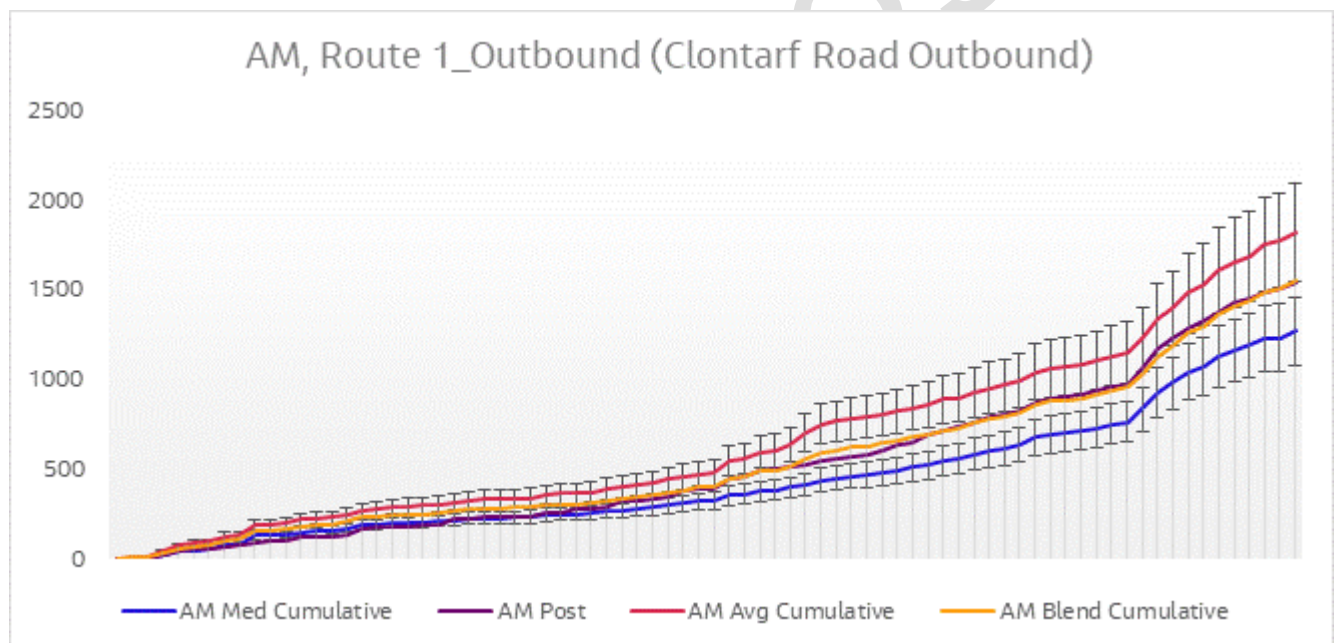
Figure 6-12 Journey Time Validation Plot - Route 1 Outbound AM
