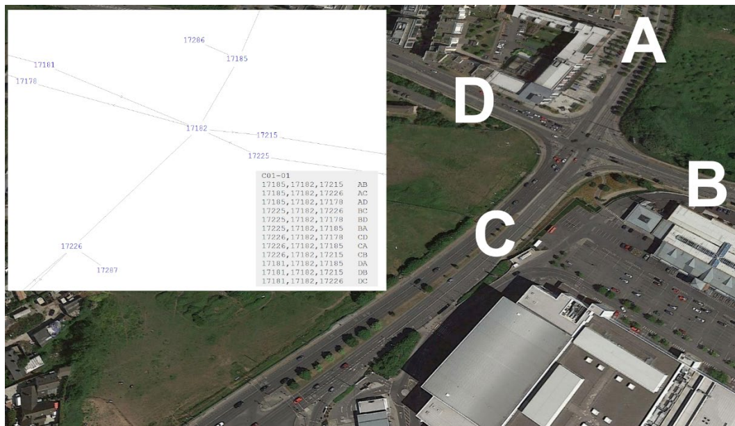
Figure 5-2 ATC and JTC Traffic counts location Bus Connects LAM Node Matching (Junction C01-01)
