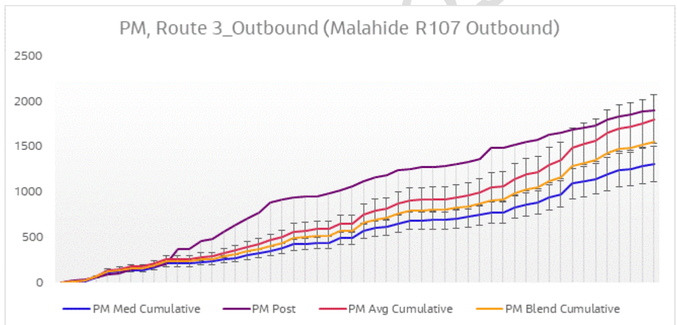
Figure 6-26 Journey Time Validation Plot - Route 3 Outbound PM
