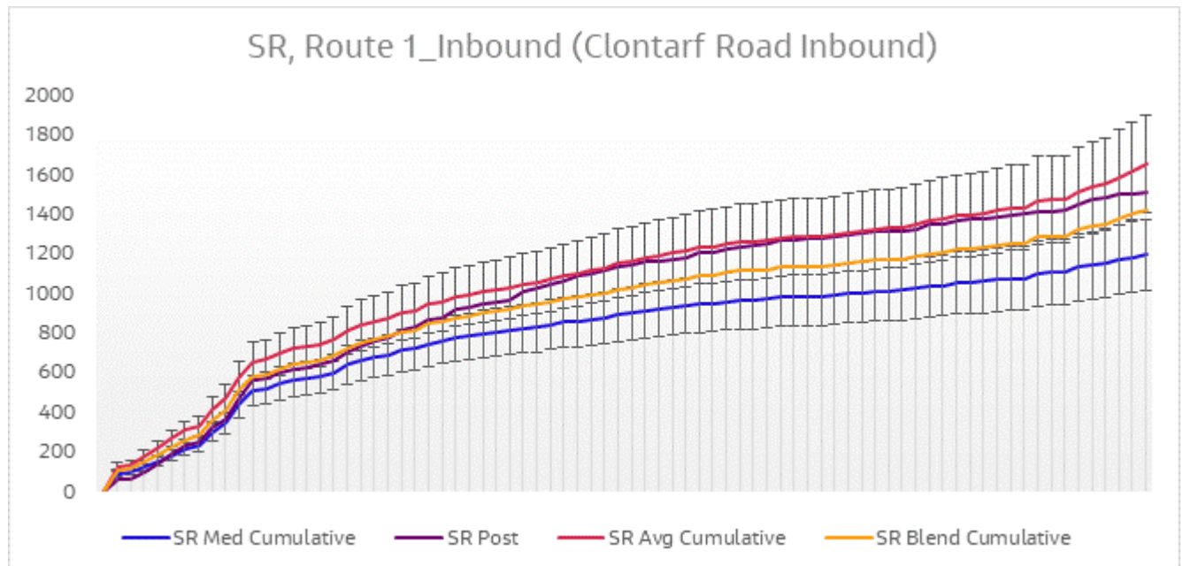
Figure 6-19 Journey Time Validation Plot - Route 1 Inbound SR
