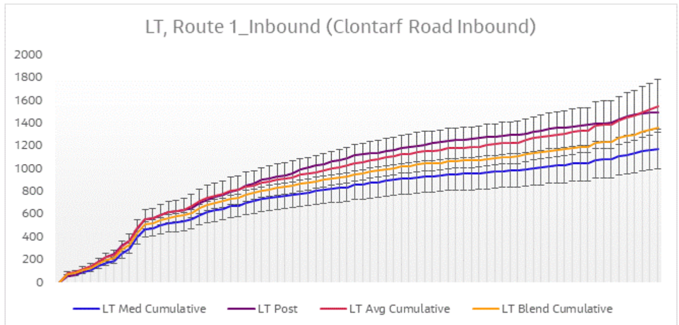
Figure 6-15 Journey Time Validation Plot - Route 1 Inbound LT
