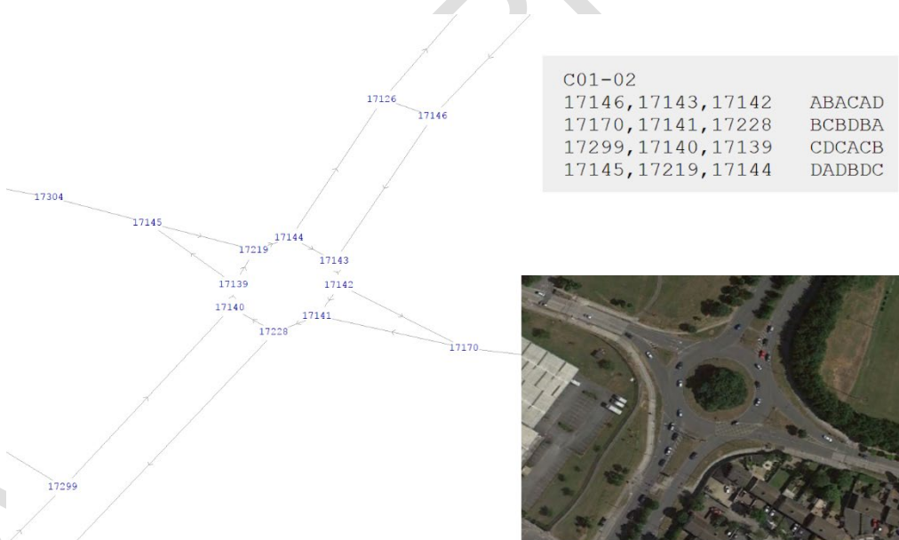
Figure 5-3 ATC and JTC Traffic counts location Bus Connects LAM Node Matching (Junction C01-02)
