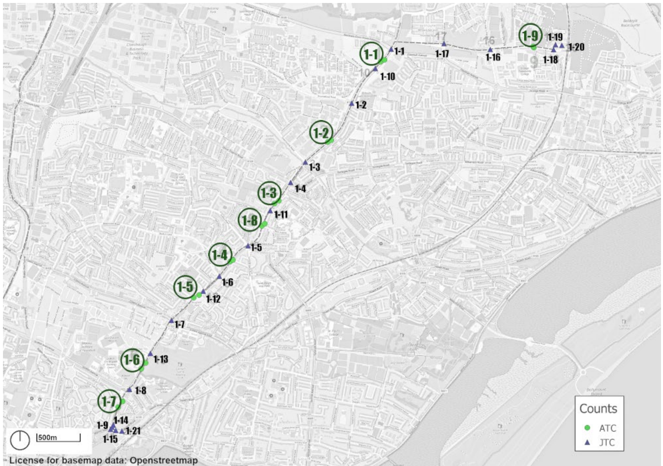
Figure 5-1 ATC and JTC Traffic counts location
