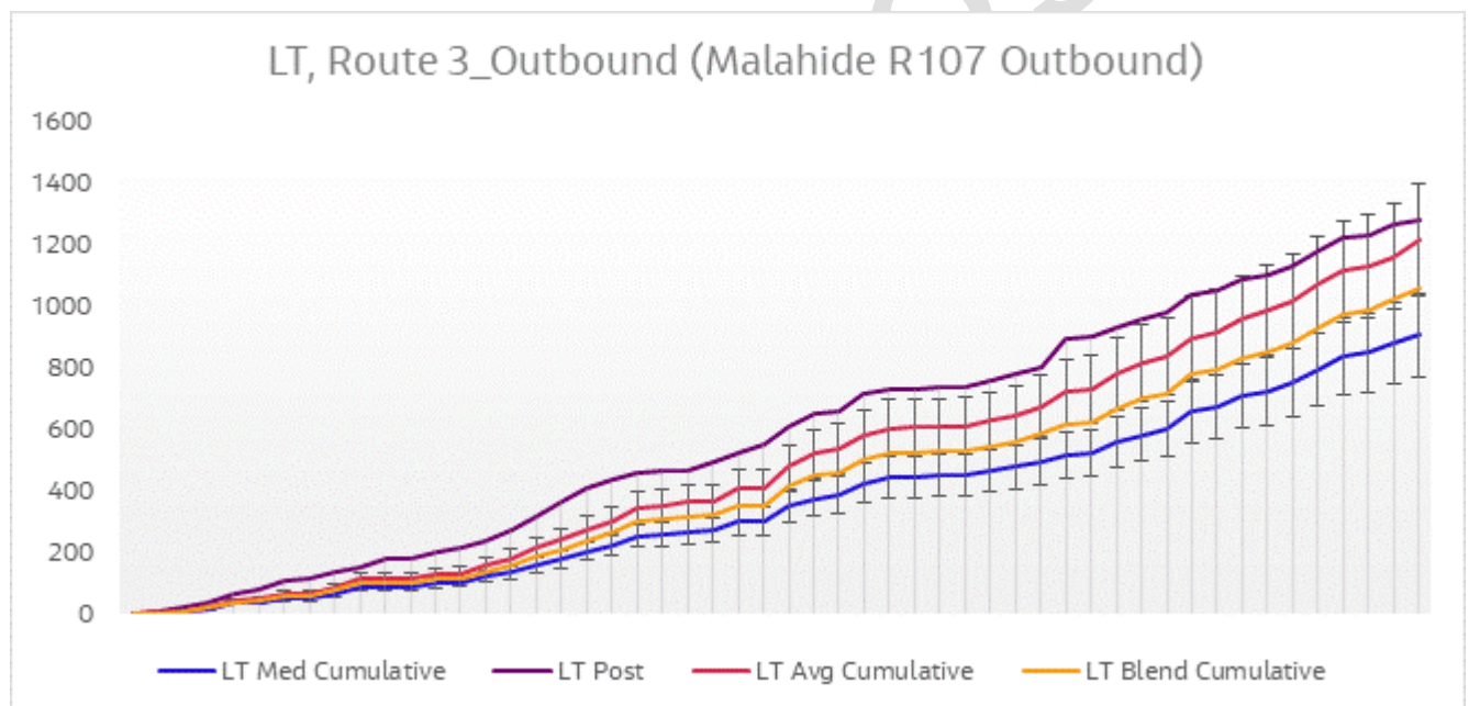
Figure 6-18 Journey Time Validation Plot - Route 3 Outbound LT
