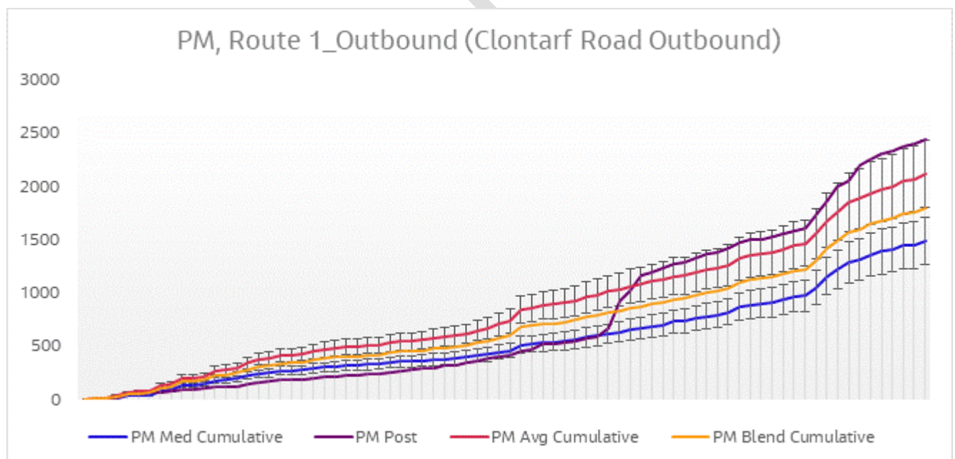
Figure 6-24 Journey Time Validation Plot - Route 1 Outbound PM
