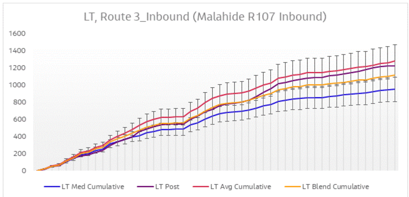
Figure 6-17 Journey Time Validation Plot - Route 3 Inbound LT
