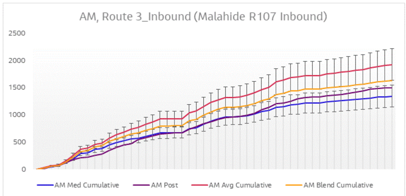
Figure 6-13 Journey Time Validation Plot - Route 3 Inbound AM
