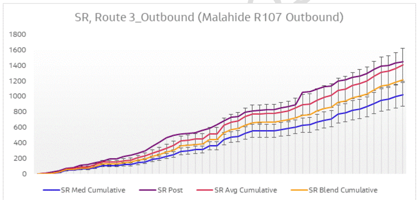
Figure 6-22 Journey Time Validation Plot - Route 3 Outbound SR
