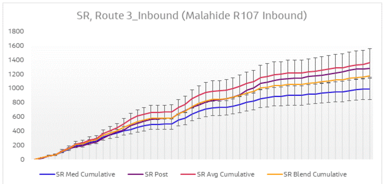
Figure 6-21 Journey Time Validation Plot - Route 3 Inbound SR
