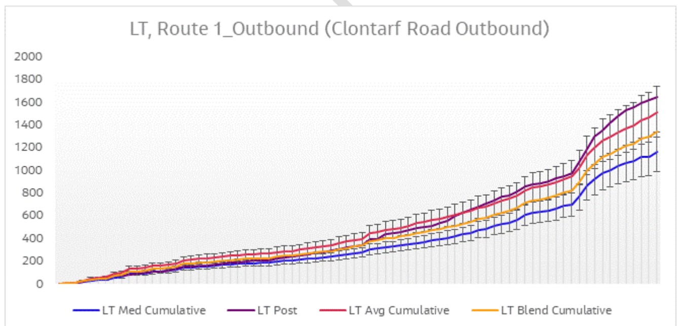
Figure 6-16 Journey Time Validation Plot - Route 1 Outbound LT
