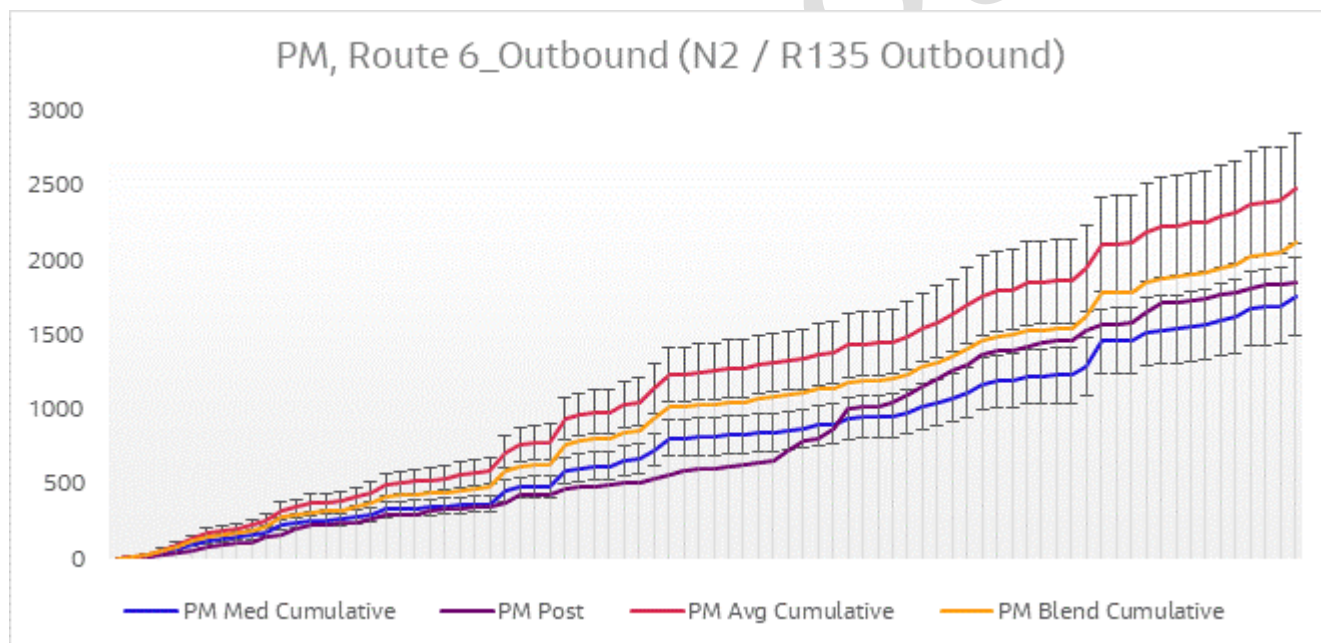
Figure 6-26 Journey Time Validation Plot - Route 6 Outbound PM
