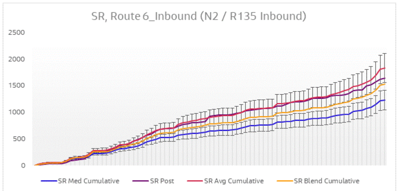
Figure 6-21 Journey Time Validation Plot - Route 6 Inbound SR
