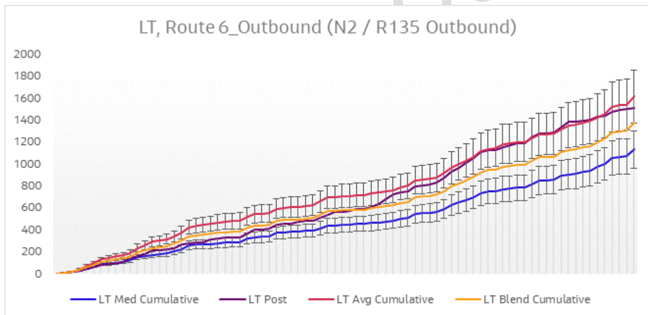
Figure 6-18 Journey Time Validation Plot - Route 6 Outbound LT
