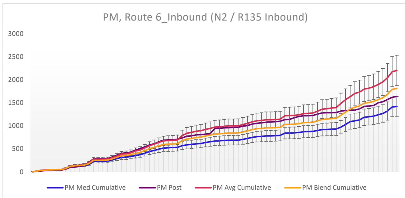
Figure 6-25 Journey Time Validation Plot - Route 6 Inbound PM
