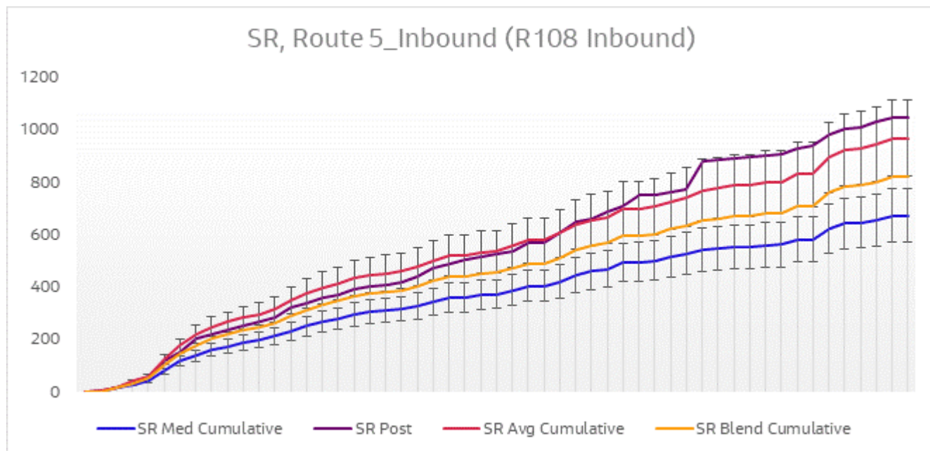
Figure 6-19 Journey Time Validation Plot - Route 5 Inbound SR
