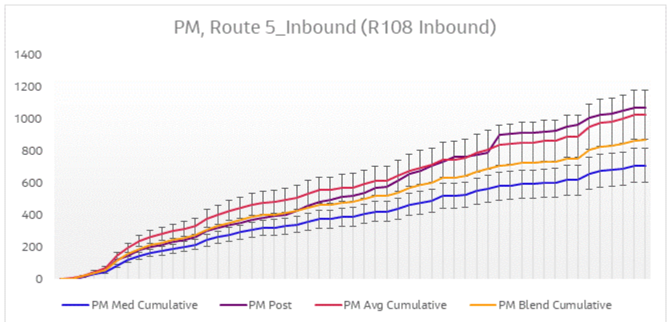
Figure 6-23 Journey Time Validation Plot - Route 5 Inbound PM
