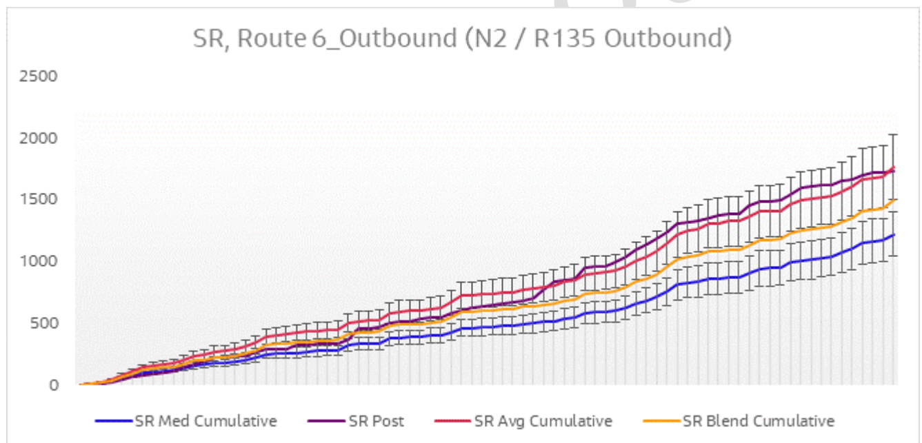
Figure 6-22 Journey Time Validation Plot - Route 6 Outbound SR
