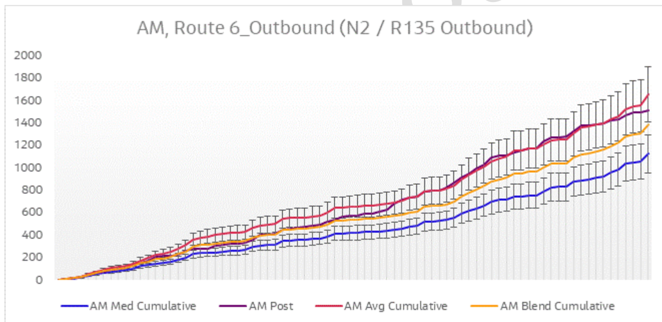
Figure 6-14 Journey Time Validation Plot – Route 6 Outbound AM
