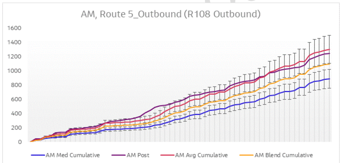
Figure 6-12 Journey Time Validation Plot - Route 5 Outbound AM
