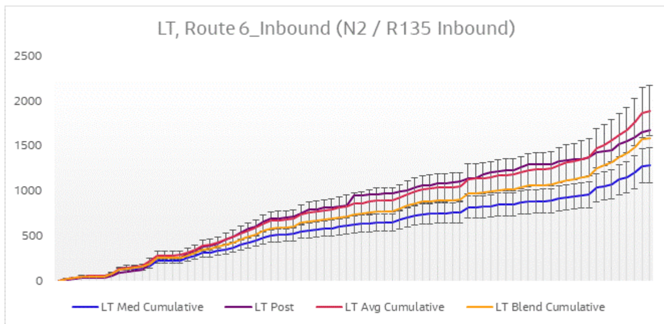
Figure 6-17 Journey Time Validation Plot - Route 6 Inbound LT
