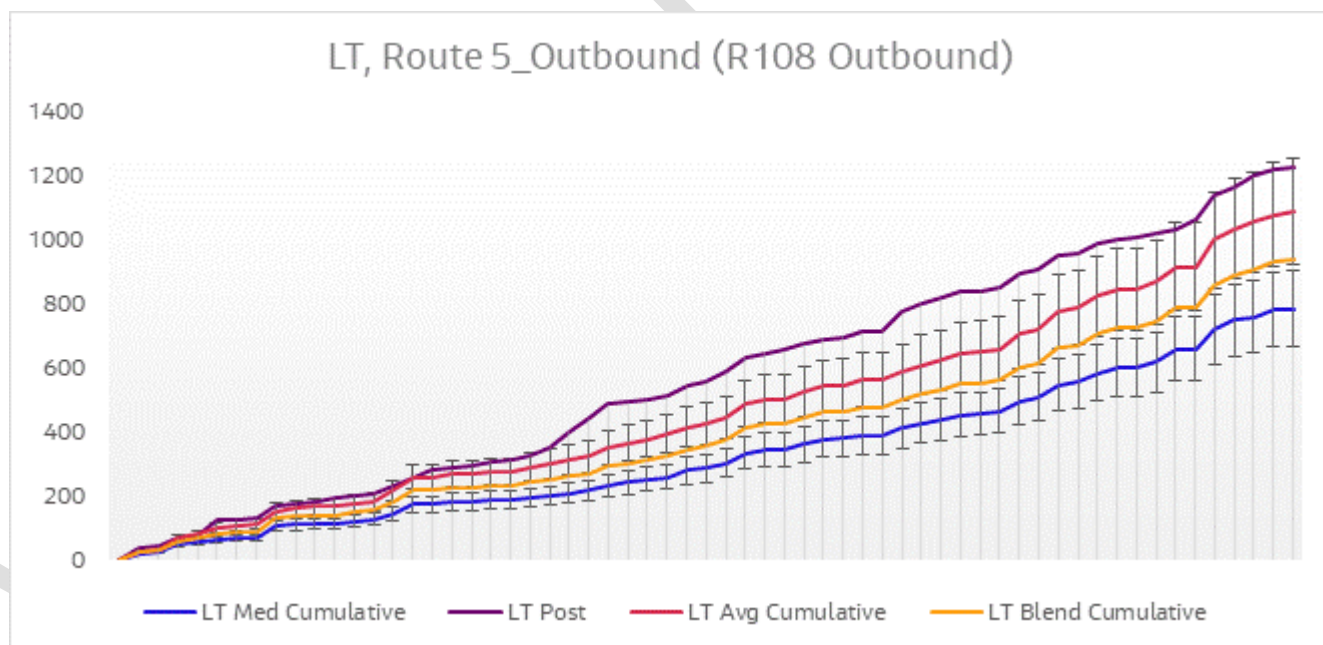
Figure 6-16 Journey Time Validation Plot - Route 5 Outbound LT
