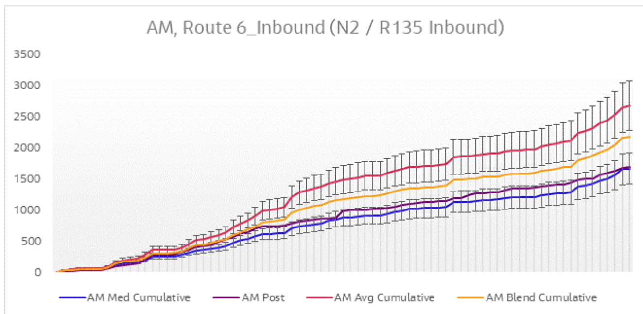
Figure 6-13 Journey Time Validation Plot - Route 6 Inbound AM
