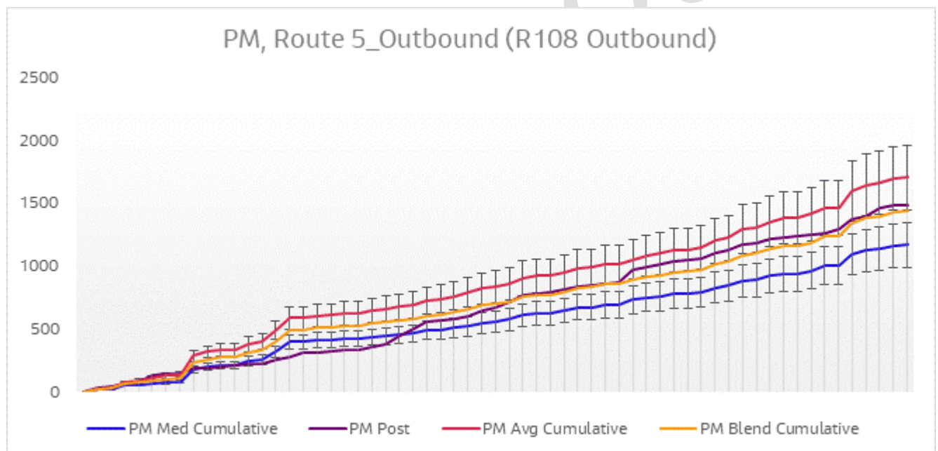
Figure 6-24 Journey Time Validation Plot - Route 5 Outbound PM
