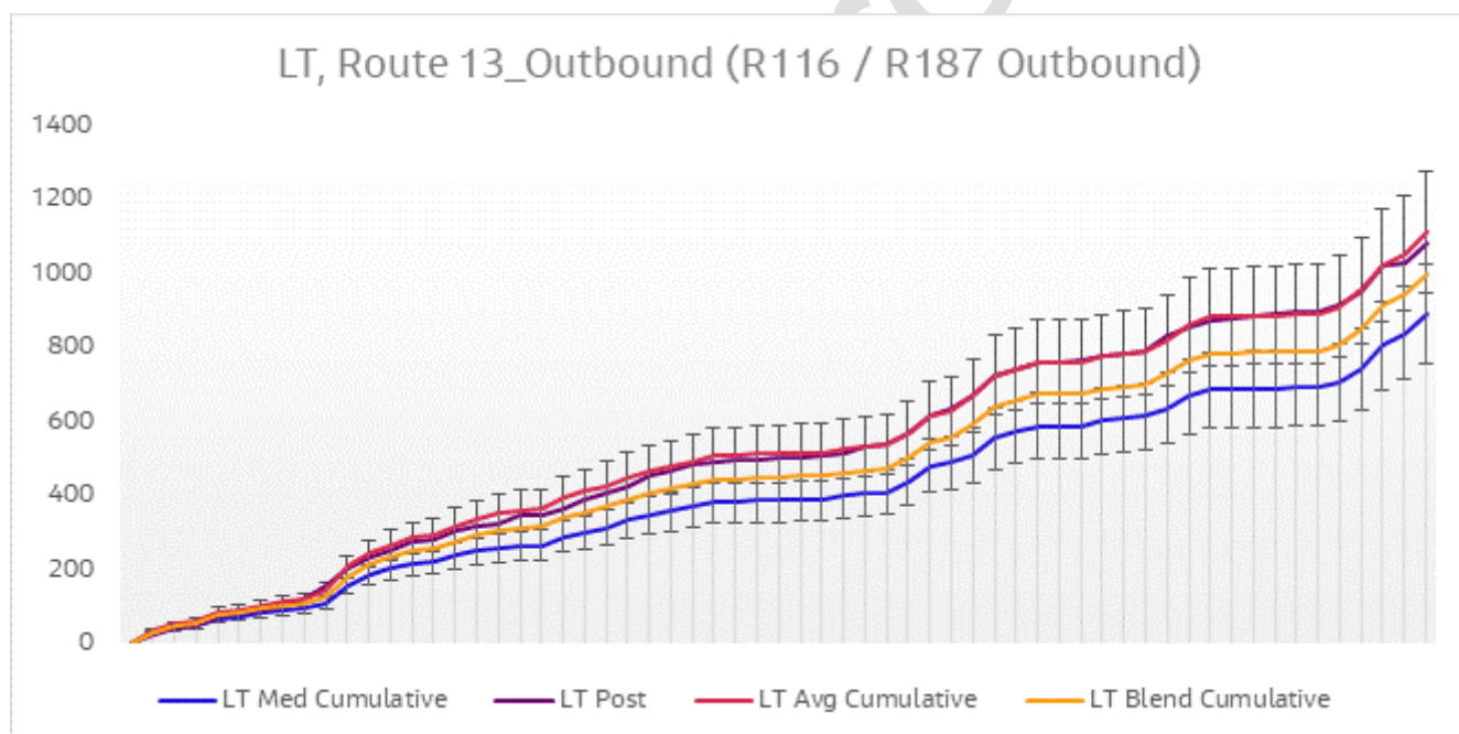
Figure 6.18 Journey Time Validation Plot - Route 13 Outbound LT
