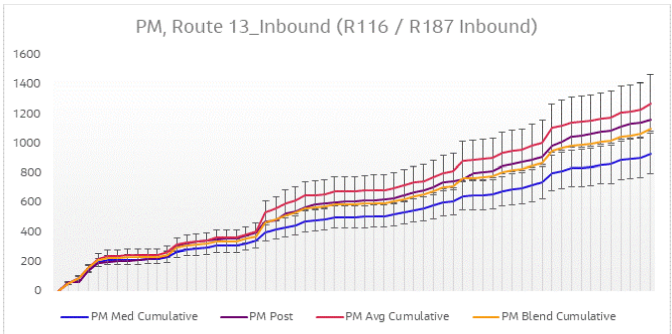
Figure 6.25 Journey Time Validation Plot - Route 13 Inbound PM
