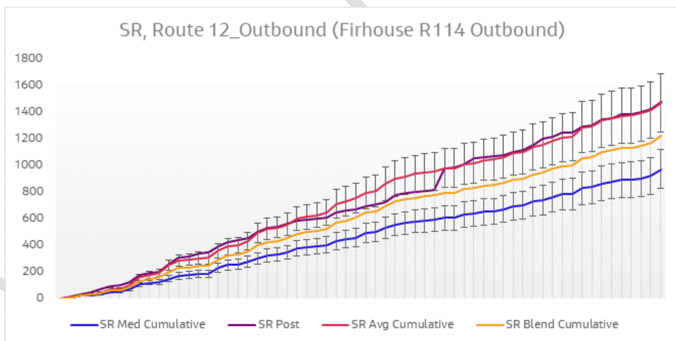
Figure 6.20 Journey Time Validation Plot - Route 12 Outbound SR
