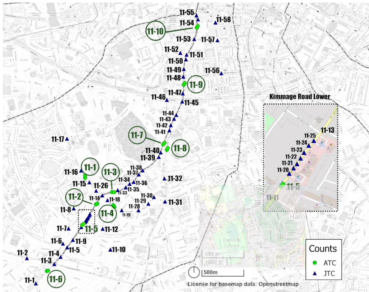
Figure 5-1 ATC and JTC Traffic counts location
