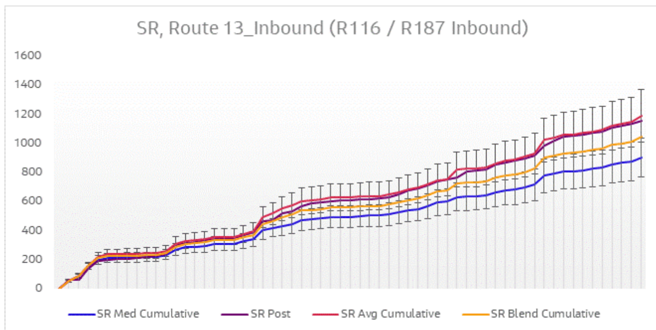
Figure 6.21 Journey Time Validation Plot - Route 13 Inbound SR
