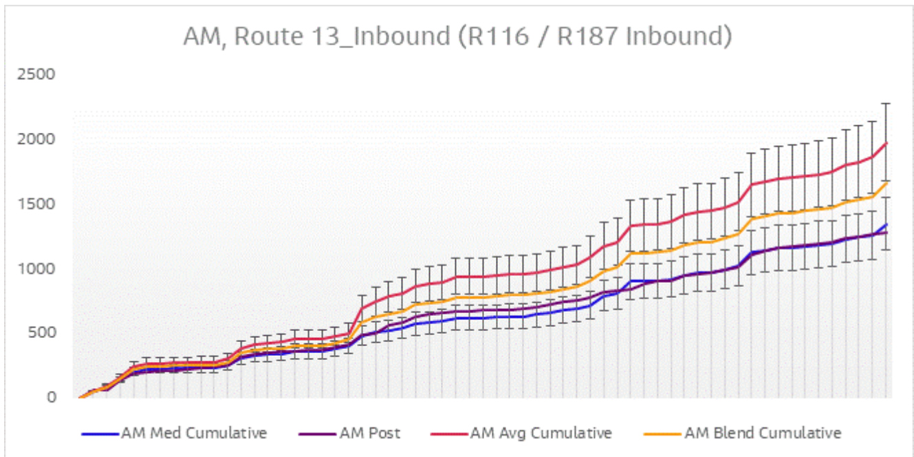
Figure 6-13 Journey Time Validation Plot - Route 13 Inbound AM
