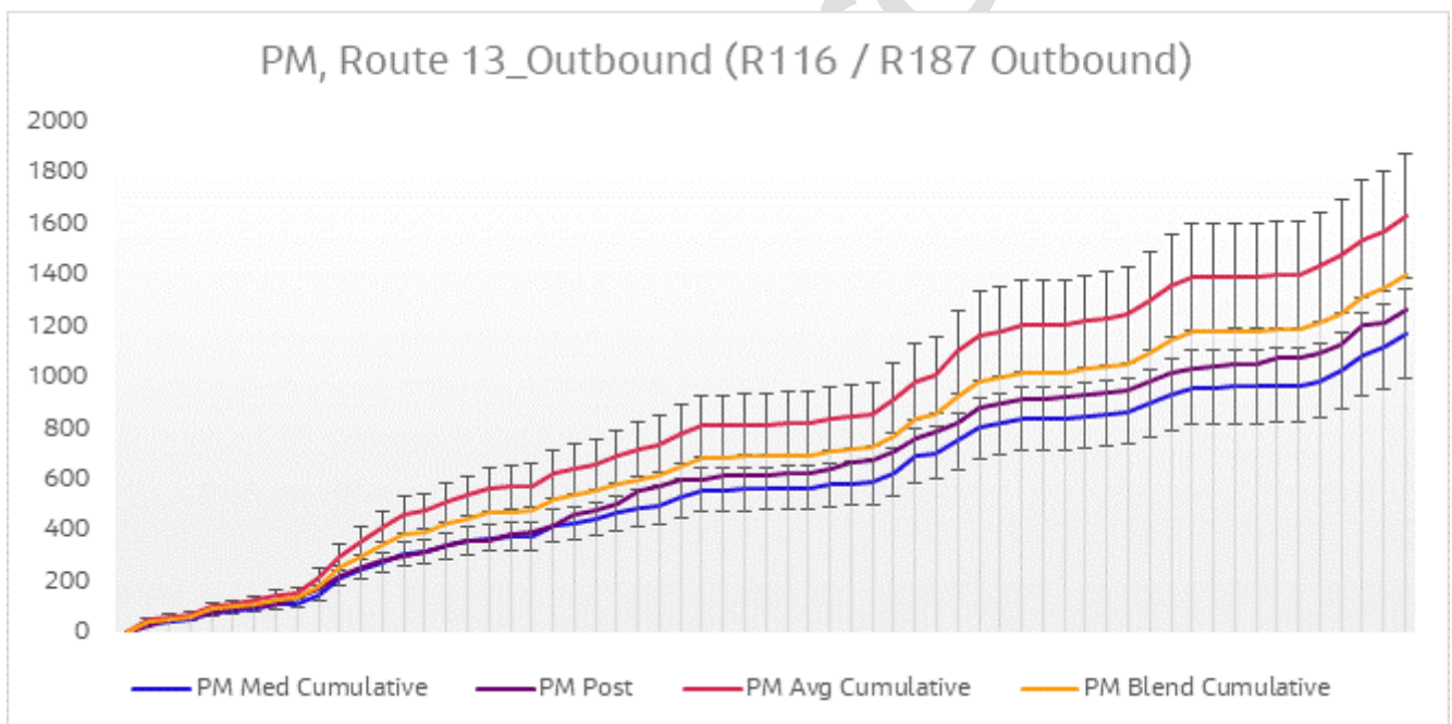
Figure 6.26 Journey Time Validation Plot - Route 13 Outbound PM
