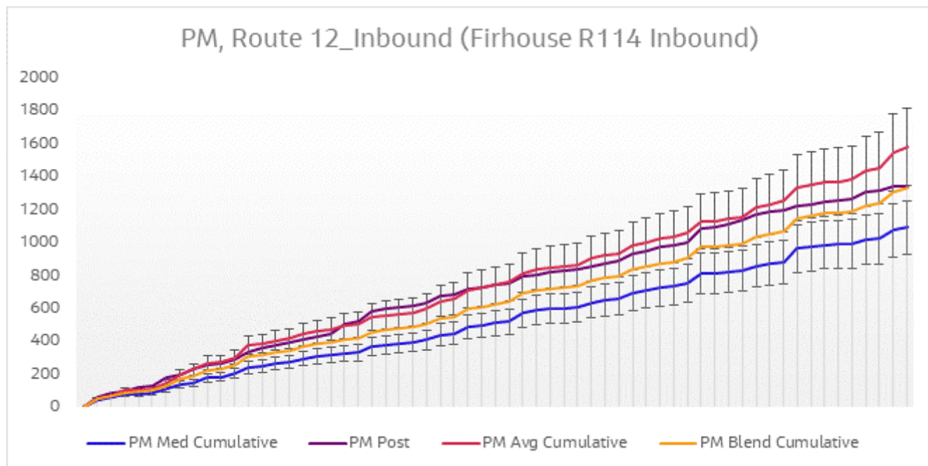
Figure 6.23 Journey Time Validation Plot - Route 12 Inbound PM
