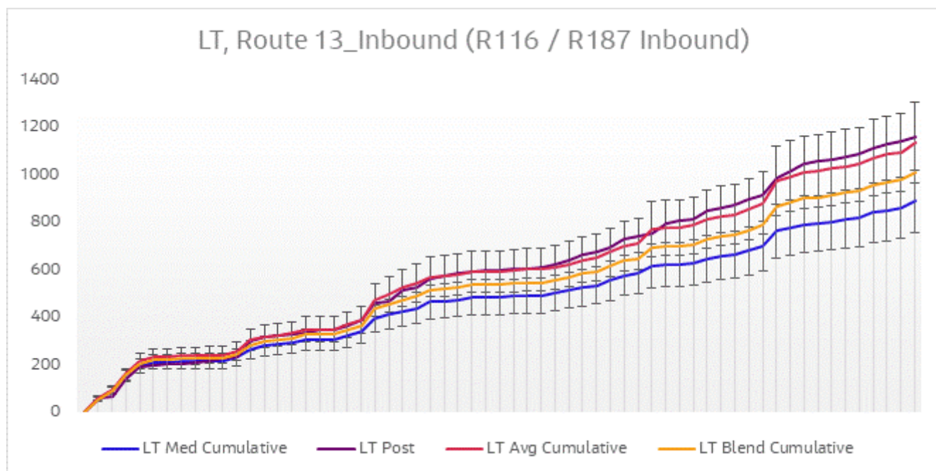
Figure 6.17 Journey Time Validation Plot - Route 13 Inbound LT
