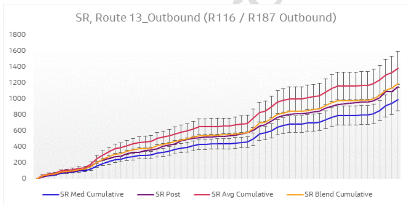
Figure 6.22 Journey Time Validation Plot - Route 13 Outbound SR
