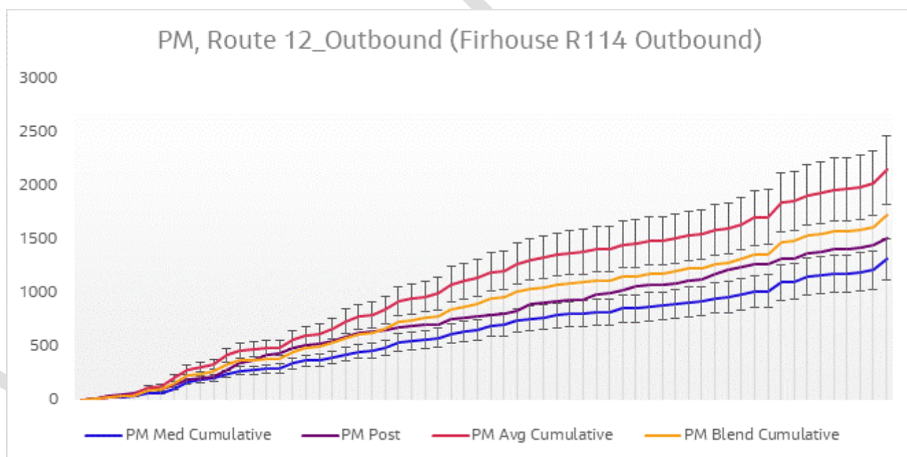
Figure 6.24 Journey Time Validation Plot - Route 12 Outbound PM
