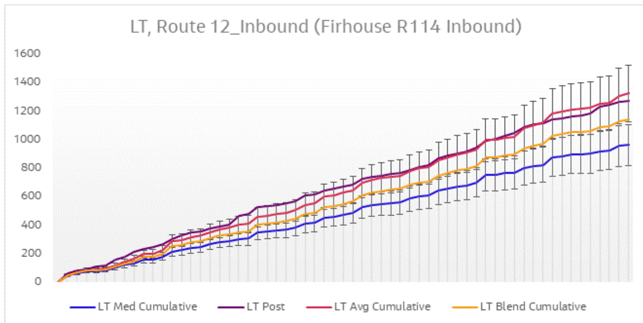
Figure 6.15 Journey Time Validation Plot - Route 12 Inbound LT
