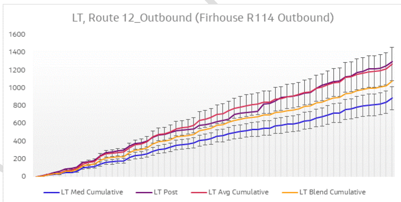
Figure 6.16 Journey Time Validation Plot - Route 12 Outbound LT
