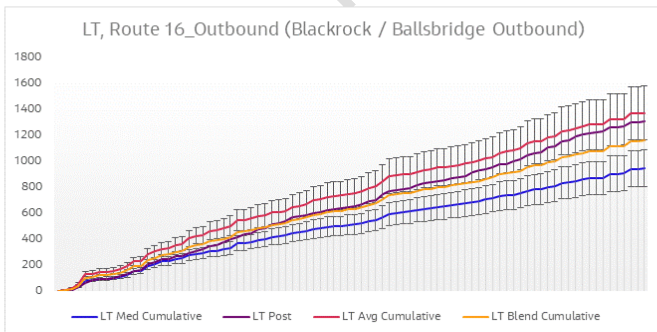
Figure 6-14 Journey Time Validation Plot - Route 16 Outbound LT
