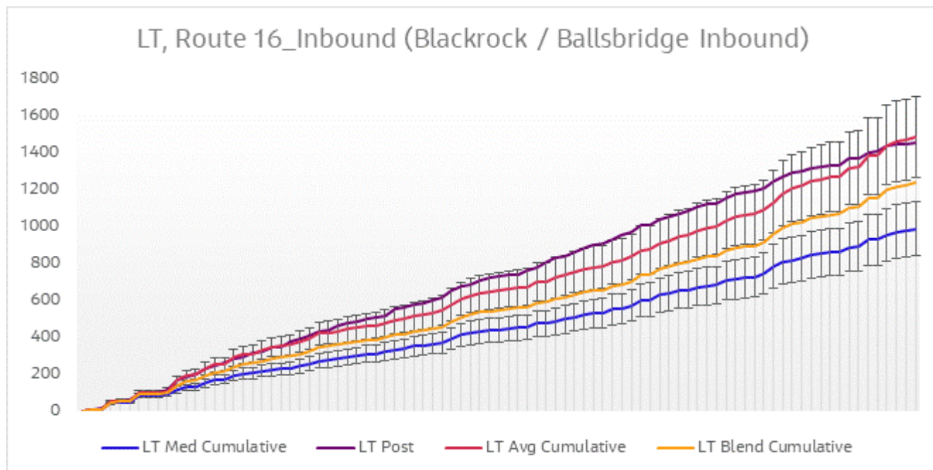
Figure 6-13 Journey Time Validation Plot - Route 16 Inbound LT
