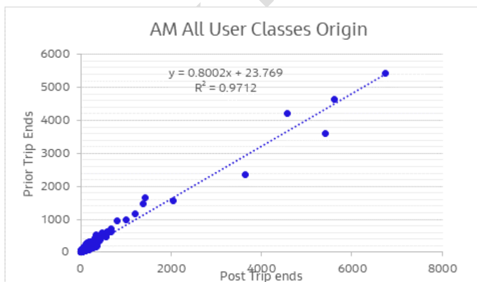
Apx Figure A-3 Regression Analysis of Matrix Estimation Changes
