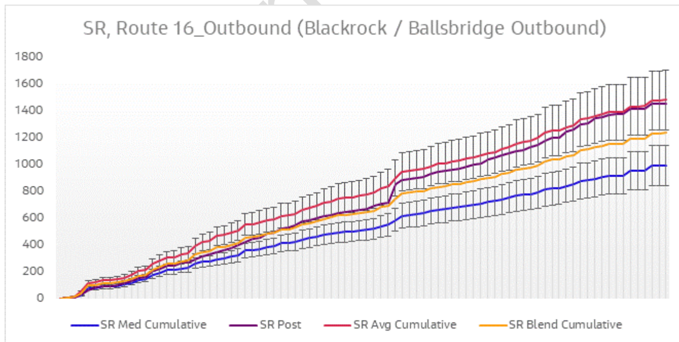
Figure 6-16 Journey Time Validation Plot - Route 16 Outbound SR
