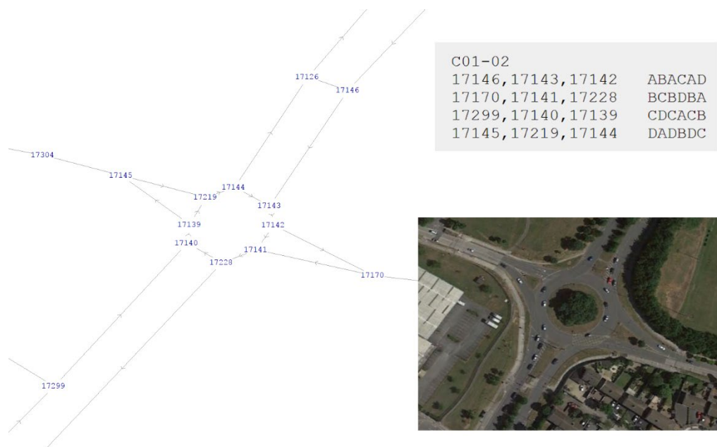
Figure 5-3 Bus Connects LAM Node Matching (Junction C01-02)
