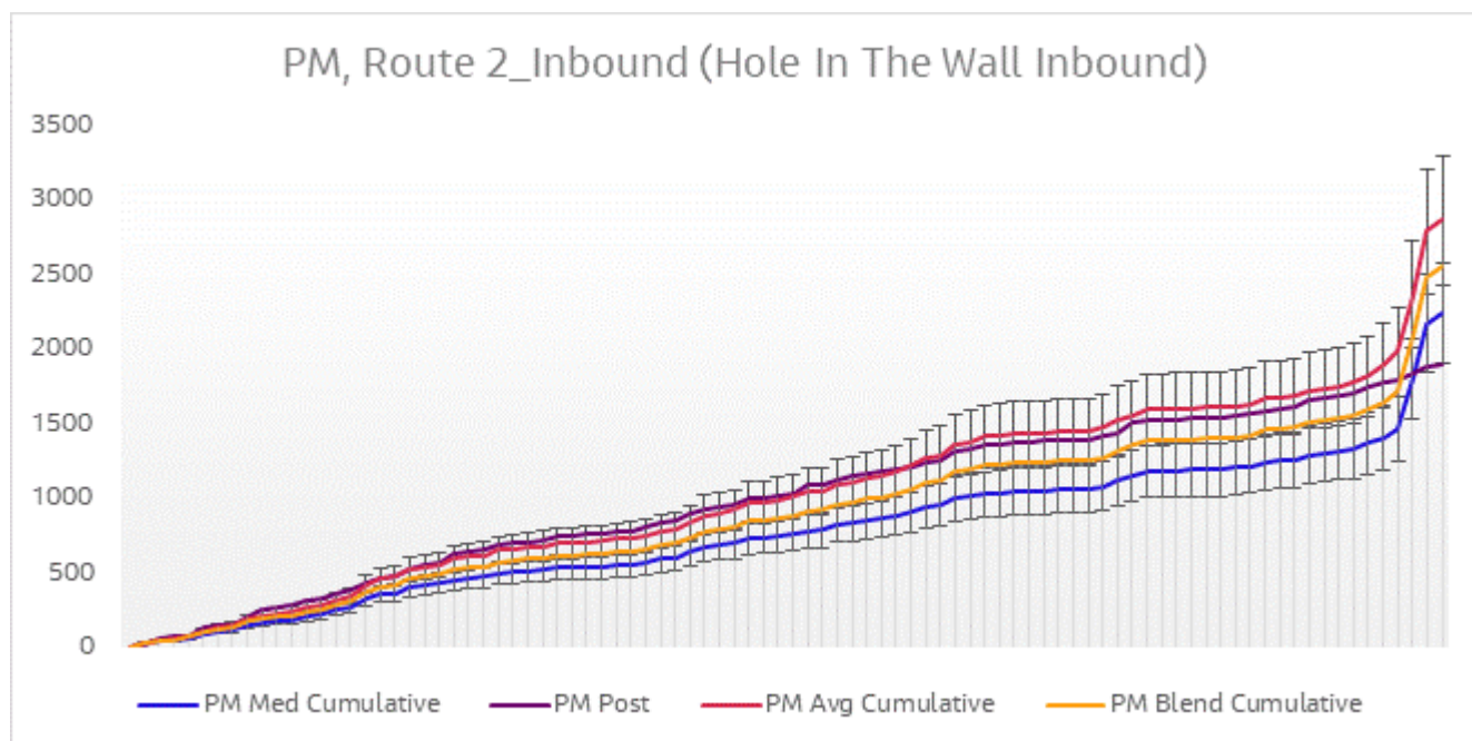
Figure 6-17 Journey Time Validation Plot - Route 2 Inbound PM
