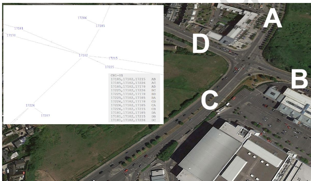
Figure 5-2 Bus Connects LAM Node Matching (Junction C01-01)
