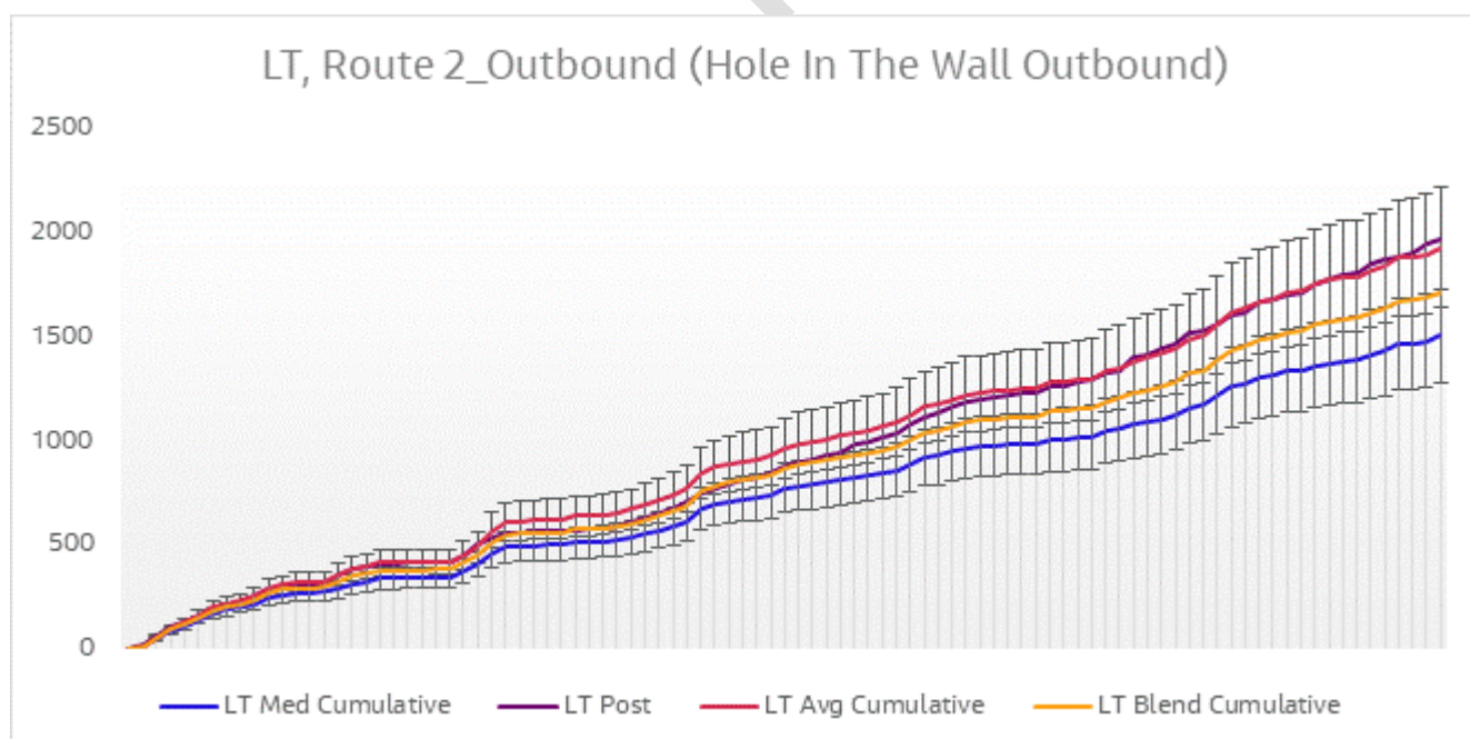
Figure 6-14 Journey Time Validation Plot - Route 2 Outbound LT
