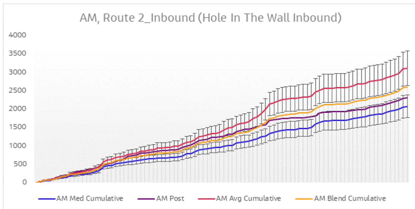
Figure 6-11 Journey Time Validation Plot - Route 2 Inbound AM
