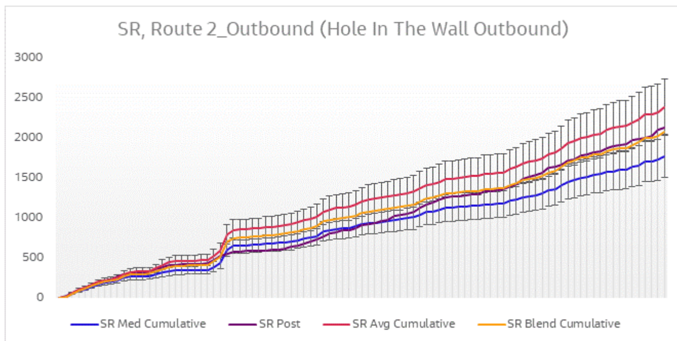
Figure 6-16 Journey Time Validation Plot - Route 2 Outbound SR
