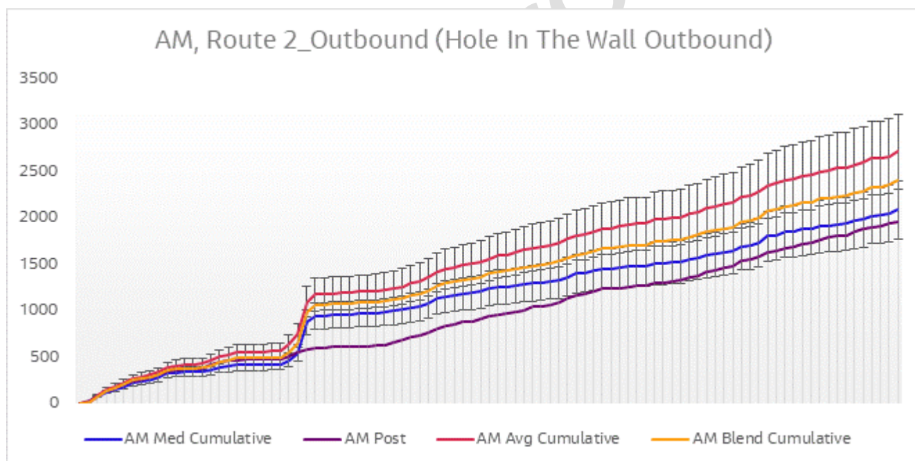
Figure 6-12 Journey Time Validation Plot - Route 2 Outbound AM
