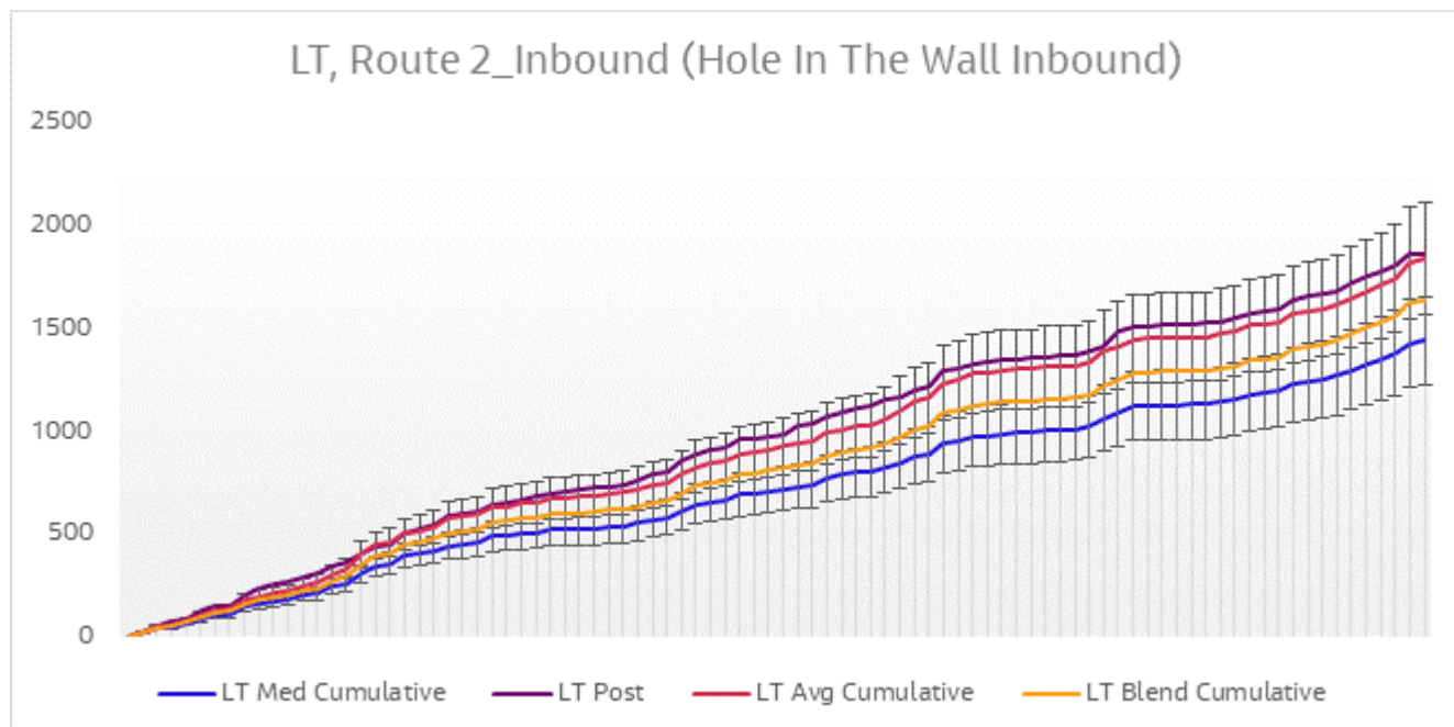
Figure 6-13 Journey Time Validation Plot - Route 2 Inbound LT
