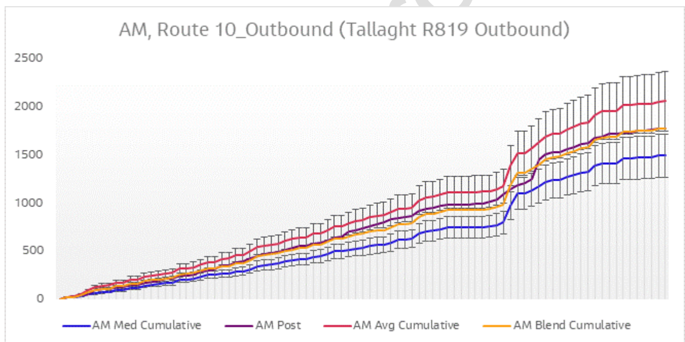
Figure 6-12 Journey Time Validation Plot - Route 10 Outbound AM
