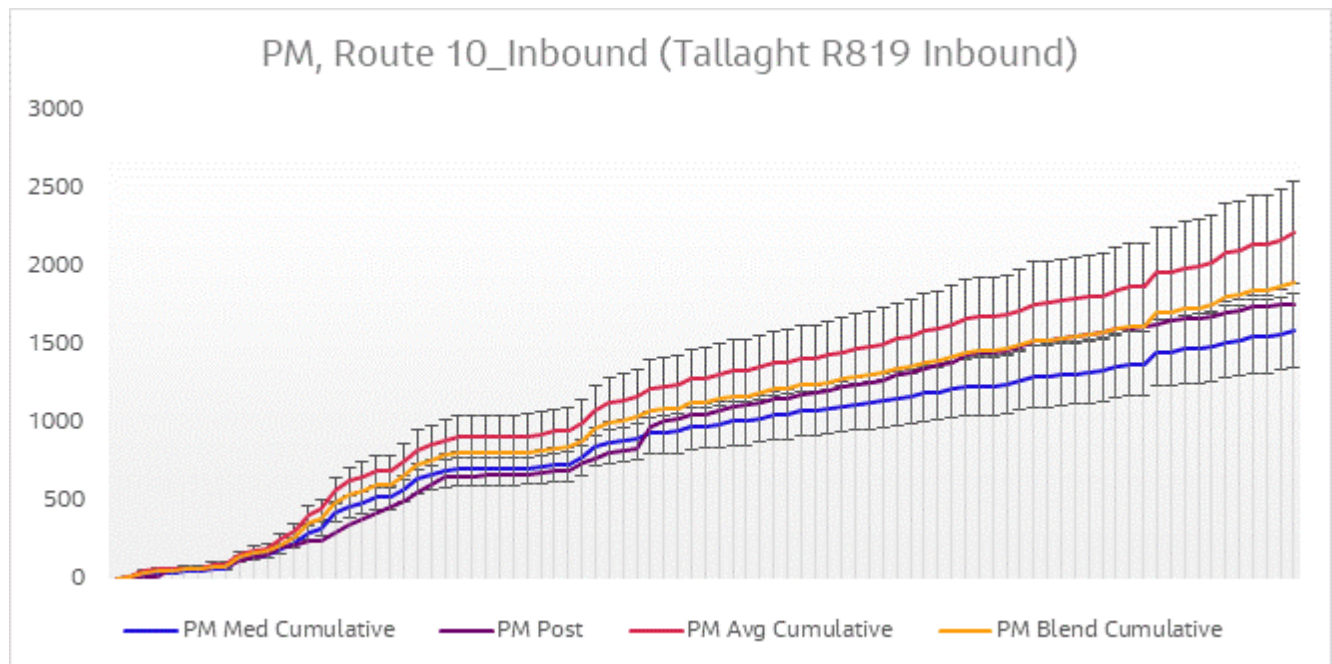
Figure 6-18 Journey Time Validation Plot - Route 10 Inbound PM
