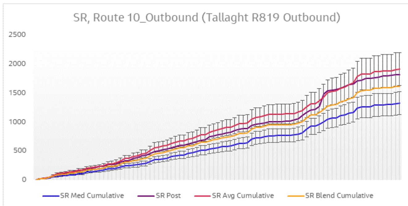
Figure 6-17 Journey Time Validation Plot - Route 10 Outbound SR
