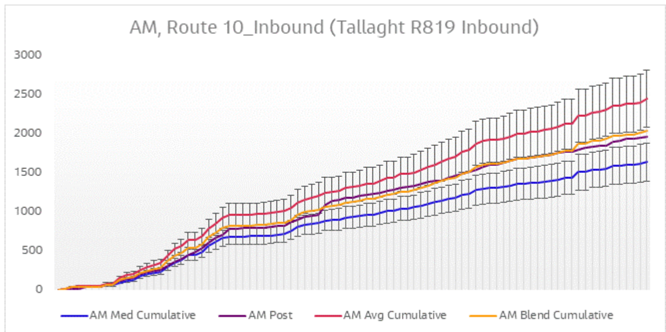
Figure 6-11 Journey Time Validation Plot - Route 10 Inbound AM
