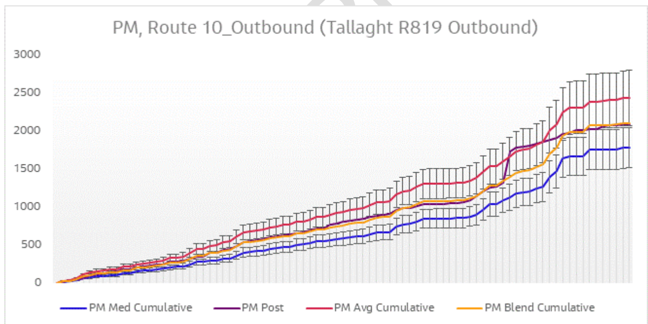
Figure 6-19 Journey Time Validation Plot - Route 10 Outbound PM
