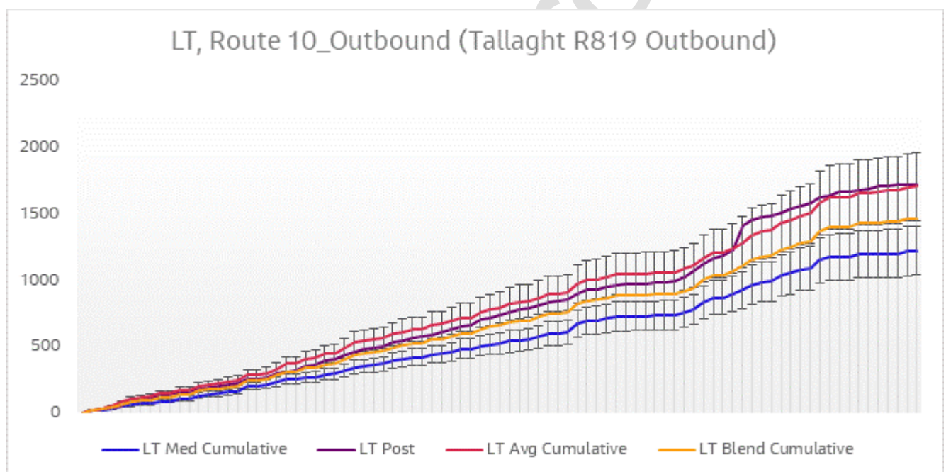
Figure 6-145 Journey Time Validation Plot - Route 10 Outbound LT
