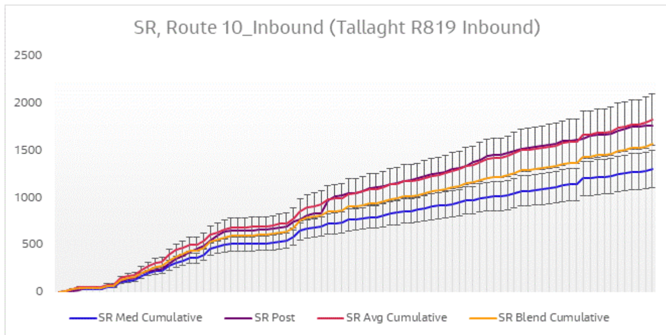
Figure 6-16 Journey Time Validation Plot - Route 10 Inbound SR
