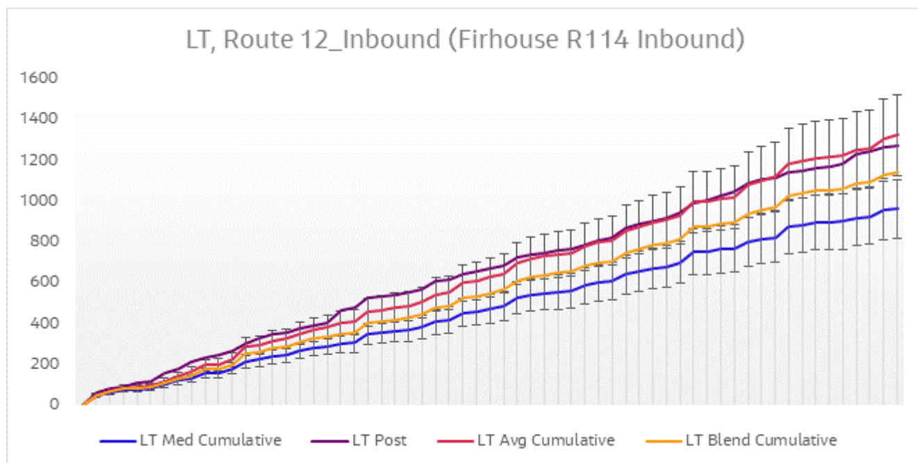
Figure 6-17 Journey Time Validation Plot - Route 12 Inbound LT
