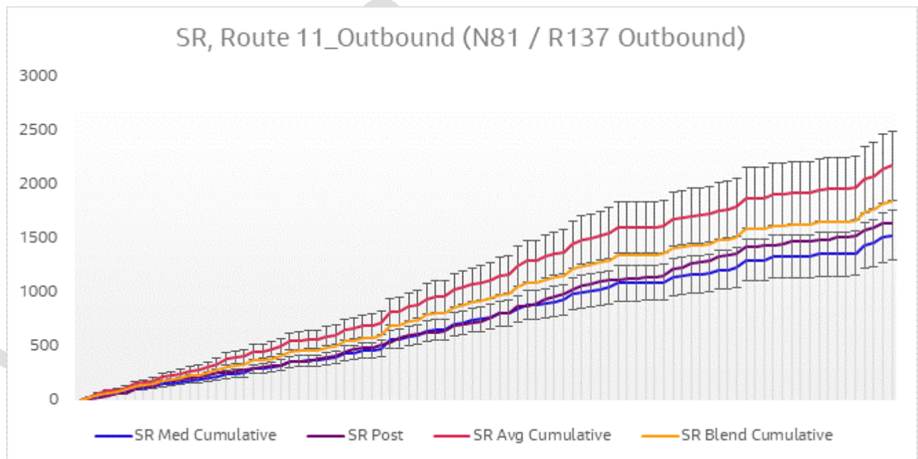
Figure 6-20 Journey Time Validation Plot - Route 11 Outbound SR
