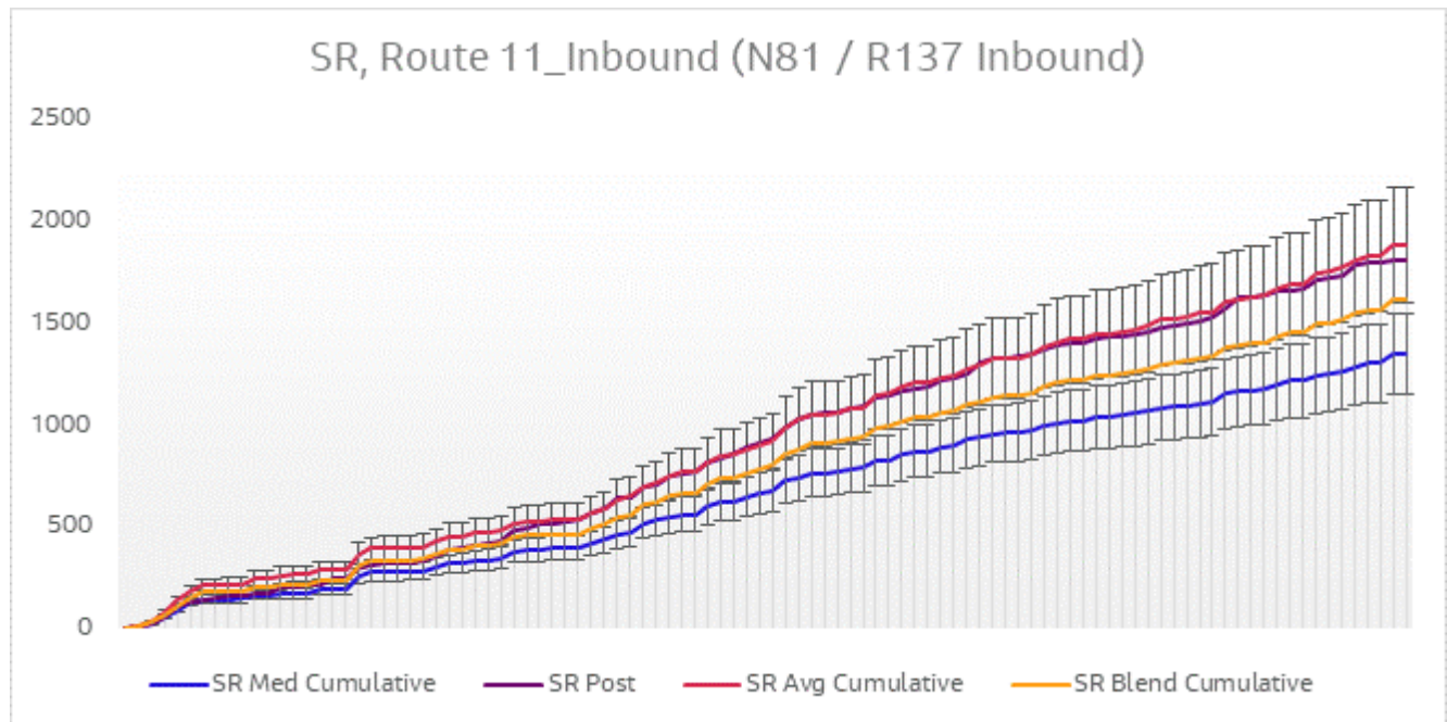
Figure 6-19 Journey Time Validation Plot - Route 11 Inbound SR
