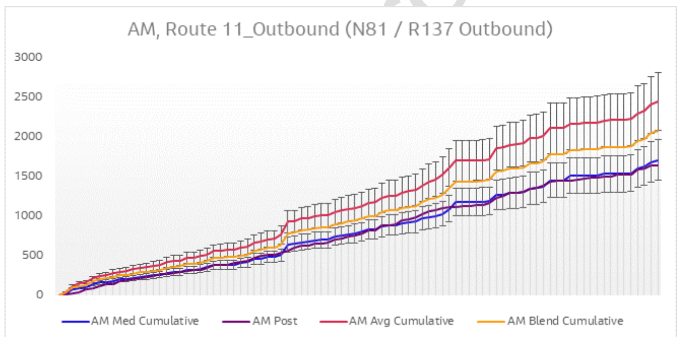
Figure 6-12 Journey Time Validation Plot - Route 11 Outbound AM
