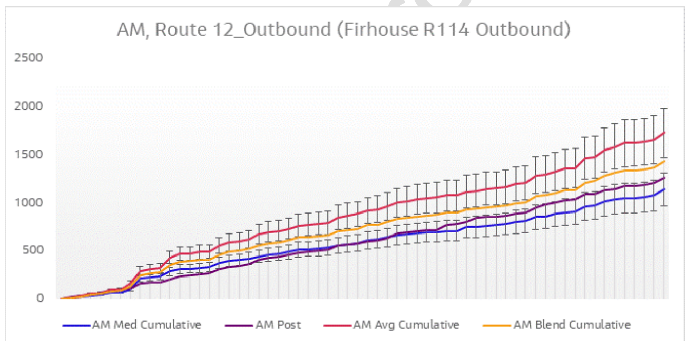
Figure 6-14 Journey Time Validation Plot - Route 12 Outbound AM
