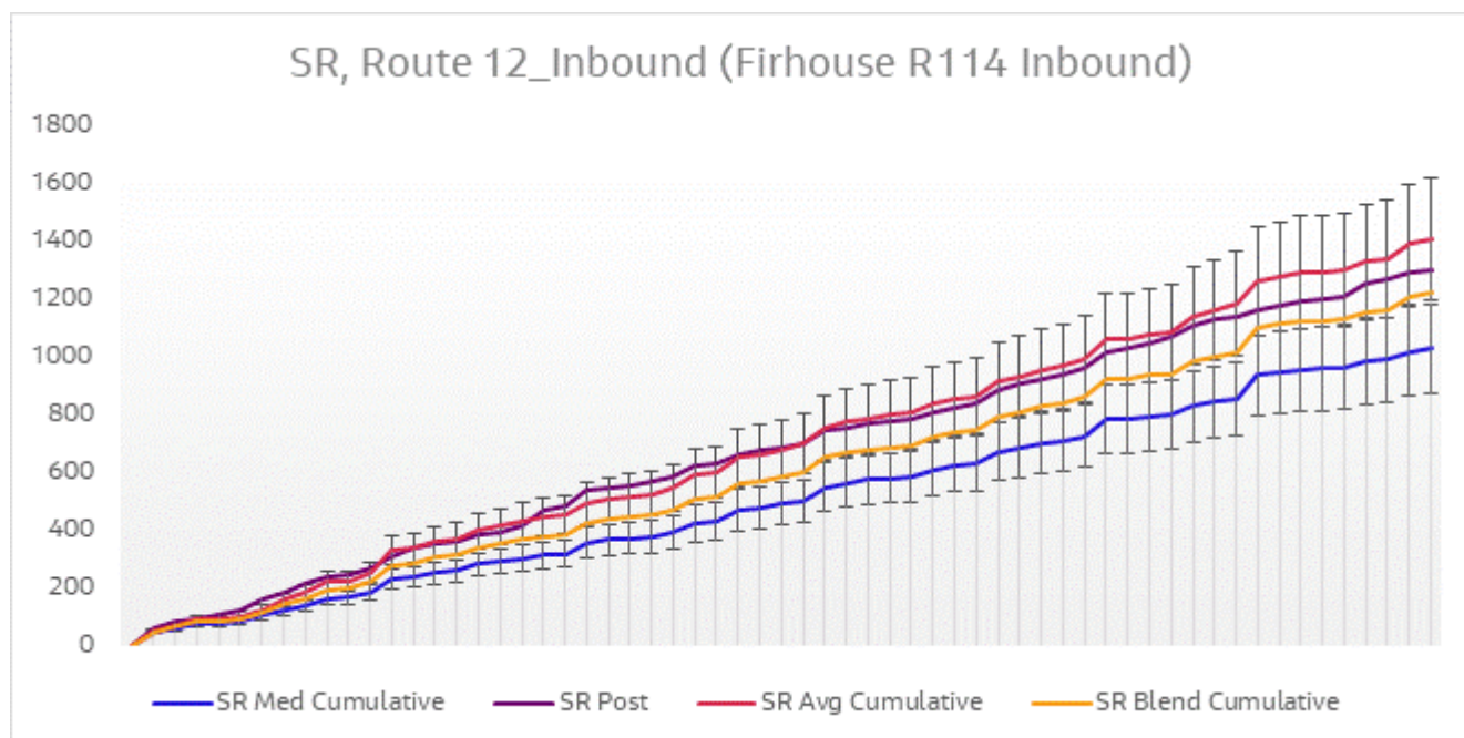
Figure 6-21 Journey Time Validation Plot - Route 12 Inbound SR
