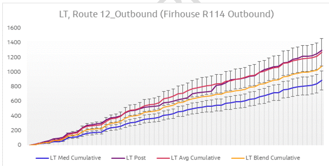
Figure 6-18 Journey Time Validation Plot - Route 12 Outbound LT
