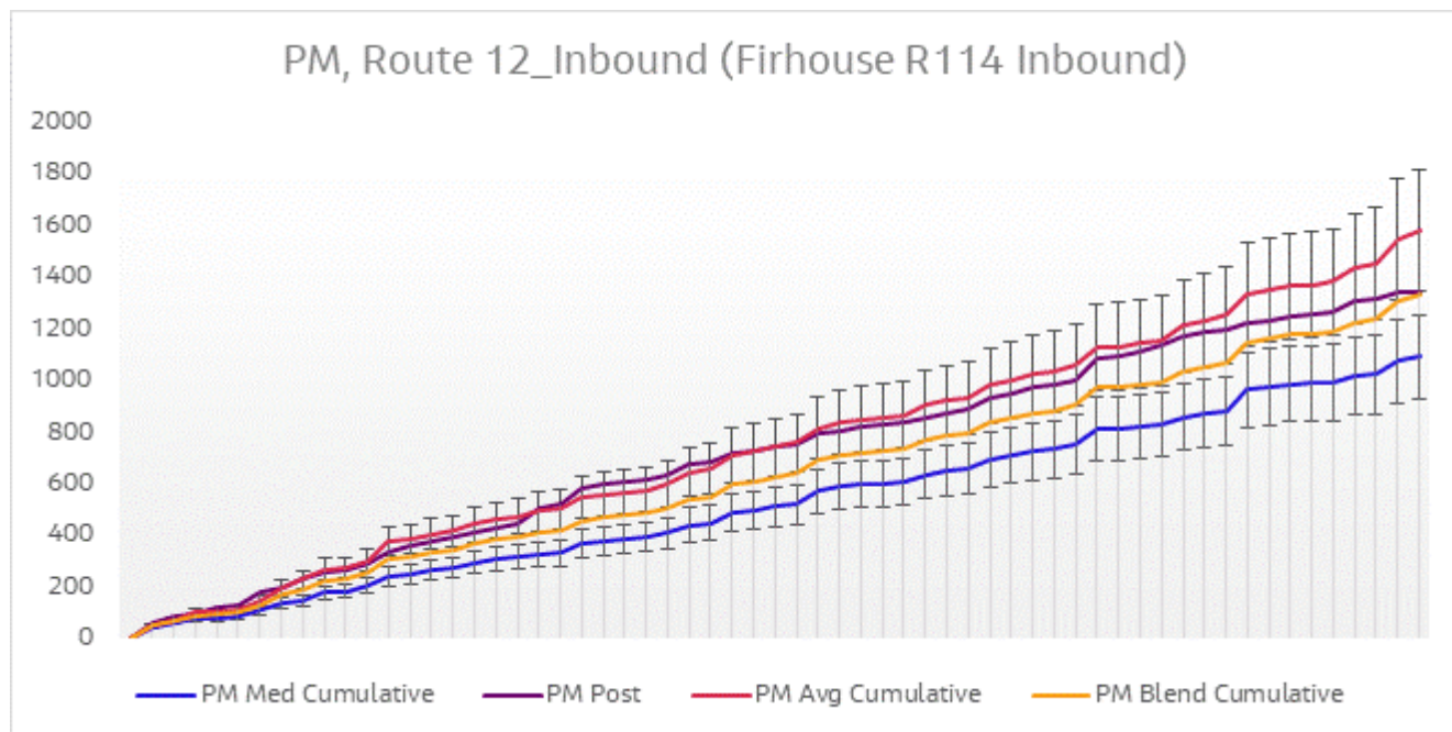
Figure 6-25 Journey Time Validation Plot - Route 12 Inbound PM
