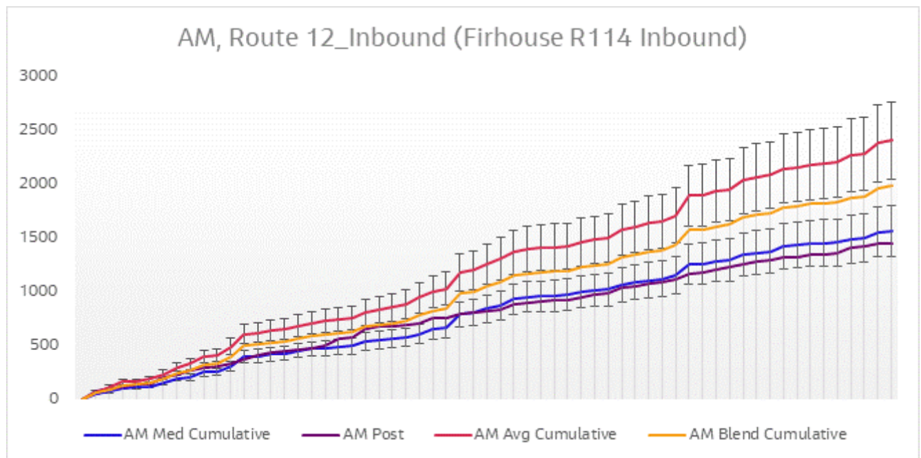
Figure 6-13 Journey Time Validation Plot - Route 12 Inbound AM
