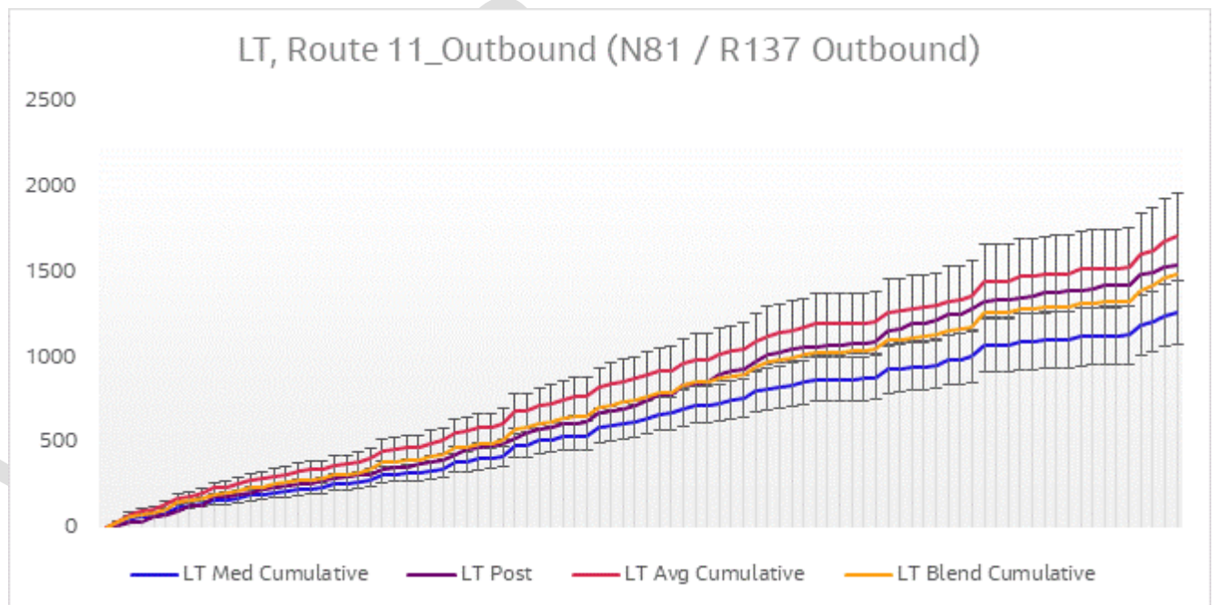
Figure 6-16 Journey Time Validation Plot - Route 11 Outbound LT
