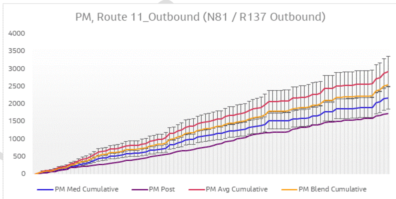
Figure 6-24 Journey Time Validation Plot - Route 11 Outbound PM
