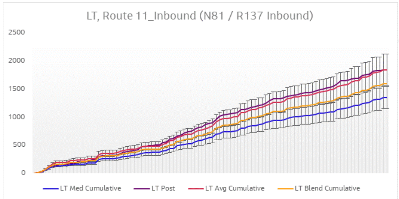
Figure 6-15 Journey Time Validation Plot - Route 11 Inbound LT
