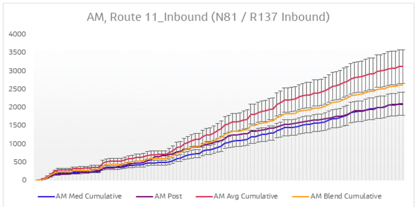
Figure 6-11 Journey Time Validation Plot - Route 11 Inbound AM
